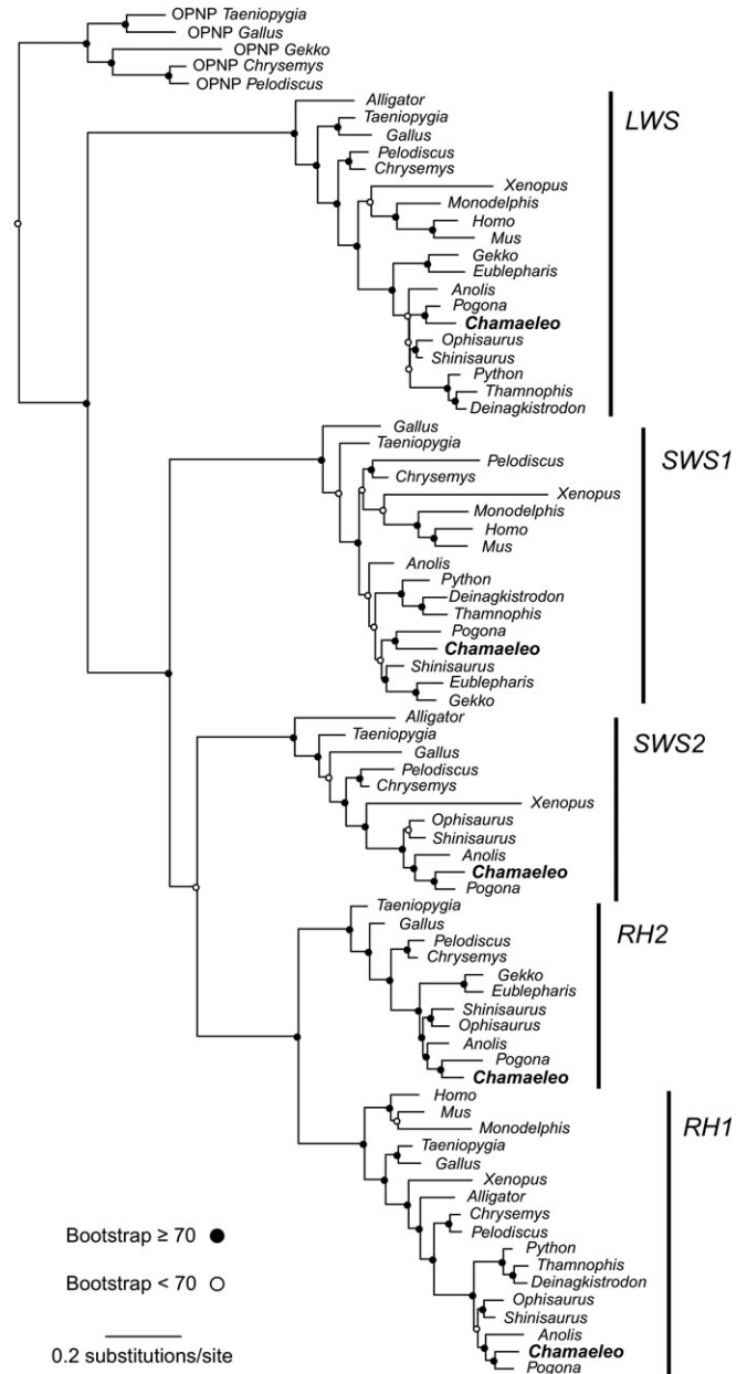
FIGURE 1 A maximum-likelihood phylogenetic reconstruction of the visual opsins of C. calyptratus and other tetrapods, including: vertebrate rhodopsin (RH1), long wavelength-sensitive opsin (LWS), short-wave sensitive 1 (SWS1), short-wave sensitive 2 (SWS2), and RH1-like 2 (RH2)
