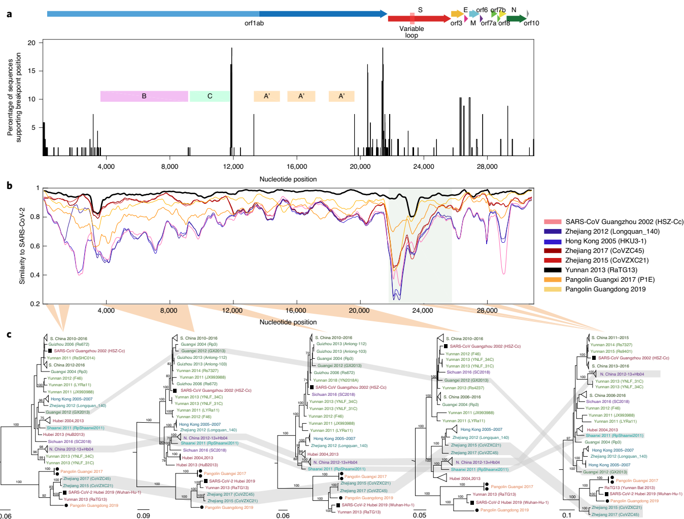
Fig. 1 | Breakpoints identified by 3SEQ. a , Breakpoints identified by 3SEQ illustrated by percentage of sequences (out of 68) that support a particular breakpoint position. Note that breakpoints can be shared between sequences if they are descendants of the same recombination events. Pink, green and orange bars show BFRs, with region A (nt 13,291–19,628) showing two trimmed segments yielding region A' (nt 13,291–14,932, 15,405–17,162, 18,009–19,628). Regions B and C span nt 3,625–9,150 and 9,261–11,795, respectively. Concatenated region A'BC is NRR1. Open reading frames are shown above the breakpoint plot, with the variable-loop region indicated in the S protein. b , Similarity plot between SARS-CoV-2 and several selected sequences including RaTG13 (black), SARS-CoV (pink) and two pangolin sequences (orange). The shaded region corresponds to the S protein. c , Maximum likelihood phylogenetic trees rooted on a 2007 virus sampled in Kenya (BtKy72; root truncated from images), shown for five BFRs of the sarbecovirus alignment. Nucleotide positions for phylogenetic inference are 147–695, 962–1,686 (first tree), 3,625–9,150 (second tree, also BFR B), 9,261–11,795 (third tree, also BFR C), 12,443–19,638 (fourth tree) and 23,631–24,633, 24,795–25,847, 27,702–28,843 and 29,574–30,650 (fifth tree). Relevant bootstrap values are shown on branches, and grey-shaded regions show sequences exhibiting phylogenetic incongruence along the genome. S. China corresponds to Guangxi, Yunnan, Guizhou and Guangdong provinces. N. China corresponds to Jilin, Shanxi, Hebei and Henan provinces, and the N. China clade also includes one sequence sampled in Hubei Province in 2004.
