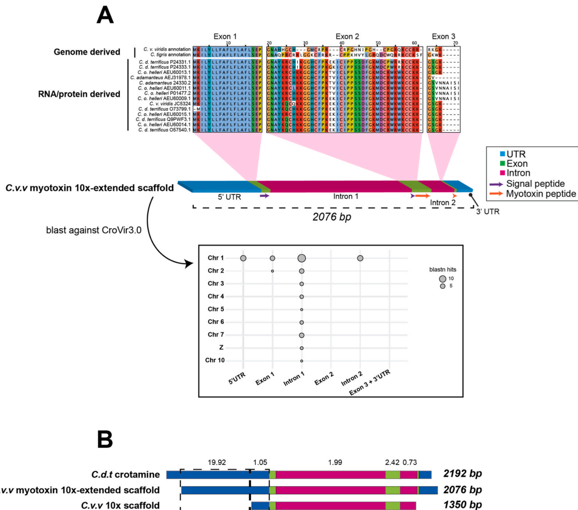
Fig. 1. Myotoxin is not present in current rattlesnake assemblies. A) A comparison of myotoxin coding sequences from Crotalus species indicates that annotated sequences from the genomes of C. tigris and C. v. viridis are not myotoxins, but rather closely related sequences. Blastn of myotoxin subsequences finds several regions of homology on chromosome 1, and other regions throughout the CroVir3.0 with homology to intron 1. B) A comparison of three independently derived inferences of myotoxin loci from a truncated 10x Genomics scaffold containing exons 1 and 2, but not 3, the paired-end read extended C. v. viridis myotoxin locus, and C. d. terrificus crotamine. Numbers above regions of the alignment indicate average pairwise Kimura-adjusted nucleotide distances, represented as differences per 100 nucleotides. Because the 5' UTR of the 10x Genomics scaffold was truncated, two separate distance comparisons were calculated. Where distances are not noted, no nucleotide differences exist across sequences.
