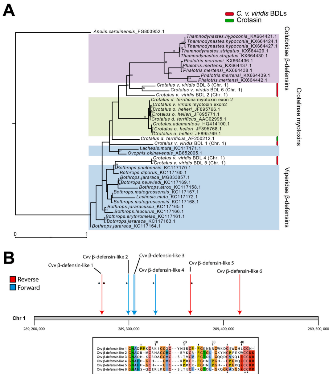
Fig. 3. β-defensin-like genes form an array on chromosome 1. A ) A rooted phylogeny of snake β-defensins, myotoxins and Cvv BDLs indicates Cvv BDLs are similar to β-defensins from both rear-fanged and front-fanged snakes. Cvv BDLs are highlighted with red bars and C. d. terrificus crostasin with a green bar. Node labels represent ultrafast bootstrap with 1000 replicates supported in over 70% of trees. Tree is rooted using a β-defensin sequence from Anolis carolinensis with homology to crostamine (Dalla Valle et al., 2012). B ) 6 β-defensin-like genes are found on chromosome 1 with signal peptides (shown as coloured dots). Exon 2 sequences are shown in the outlined box below with the conserved six-cysteine pattern labelled with asterisks.
