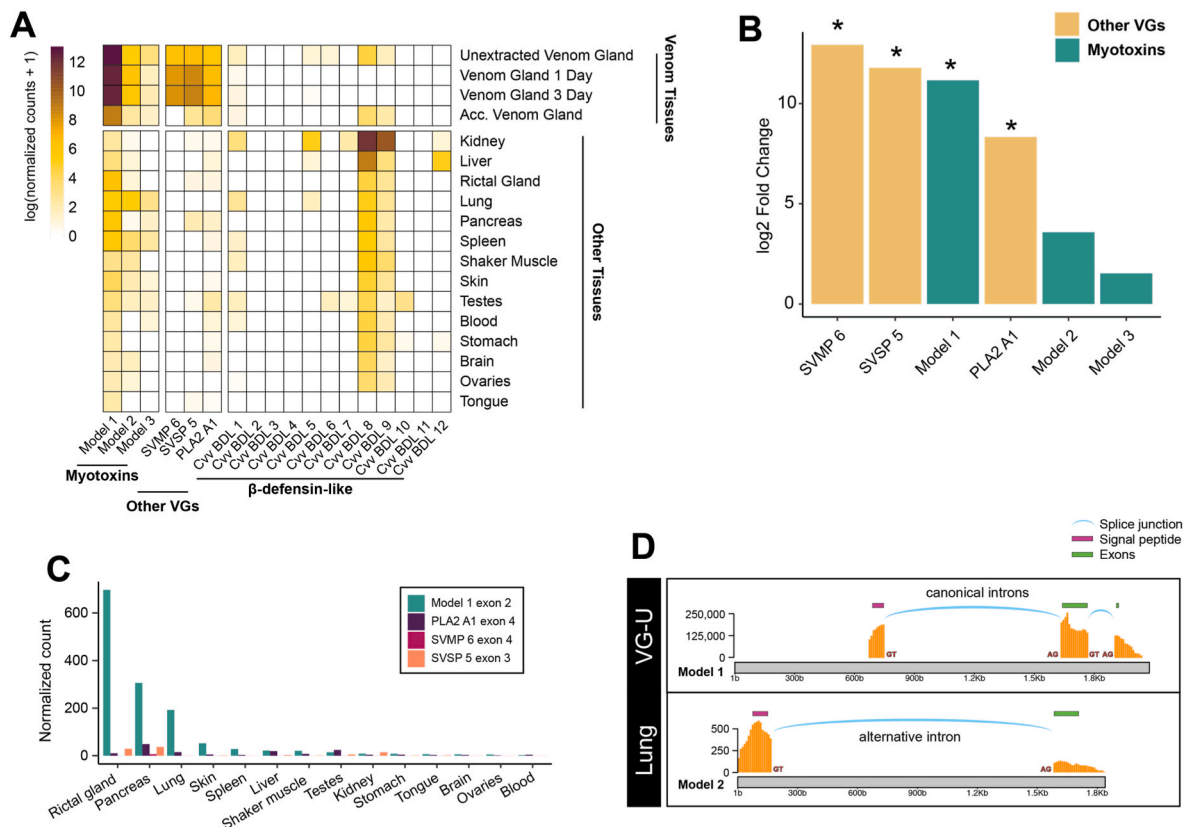
Fig. 4. RNA-seq analysis of alternative myotoxin Iso-Seq models. A) Normalized expression heatmap of three myotoxin Iso-Seq models, the three most highly expressed venom genes in C. v. viridis (Dalla Valle et al., 2012), and 12 novel C. v. viridis \beta -defensin-like genes. B) Log 2 fold change of venom associated genes shows upregulation between venom- and non-venom tissues. BH-corrected p-values < 0.05 indicated with asterisk. C) DESeq2 normalized counts of RNA reads mapped to the longest exons of venom associated genes in non-venom tissues. D) A non-canonical myotoxin RNA (Iso-Seq model 2) is spliced in lung tissue. Top panel shows canonical splicing of myotoxin in unextracted venom gland tissue. The canonical splice junction GT-AG is shown in red.
